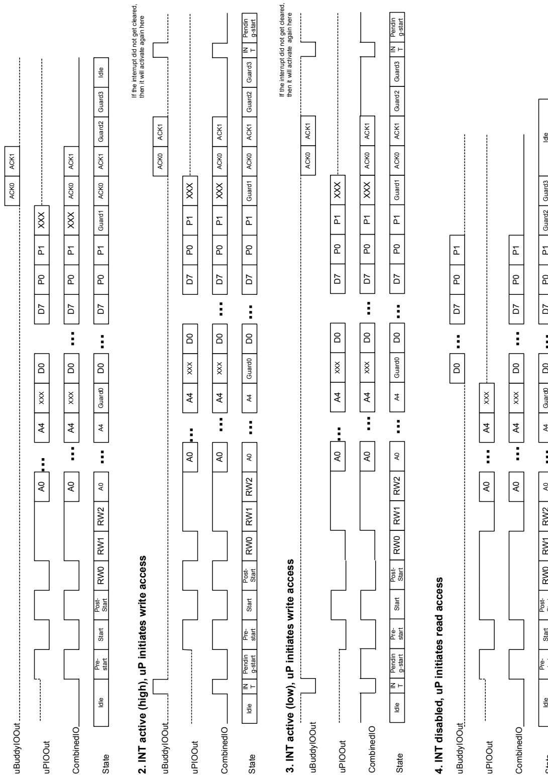
Figure 7: Serial Communication Timing Diagram
