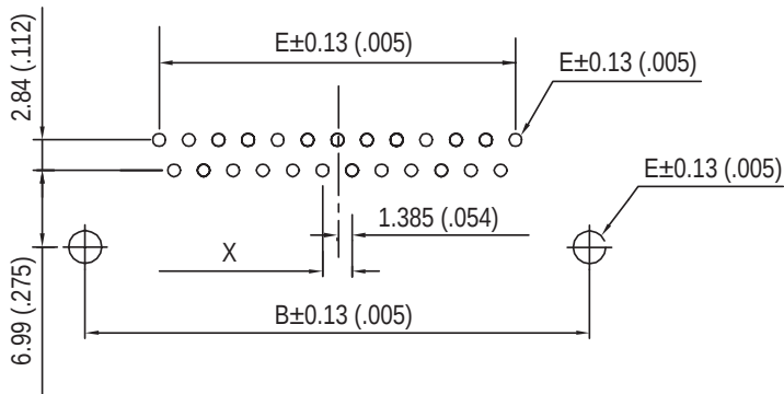
Recommended P.C.B.Layout
