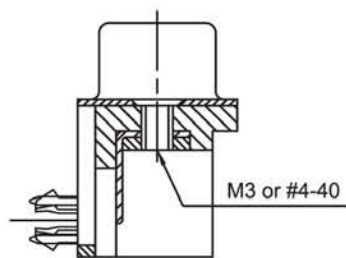
Threaded Rear Insert
