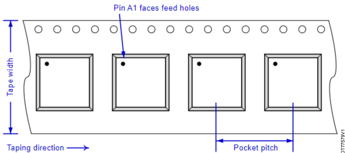
Figure 19. Carrier tape drawing with part orientation
