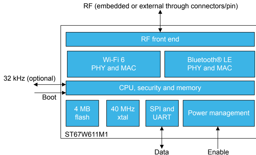
Figure 1. ST67W611M1 block diagram
