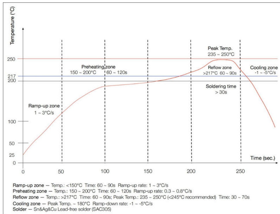
Figure 18. Soldering guideline
