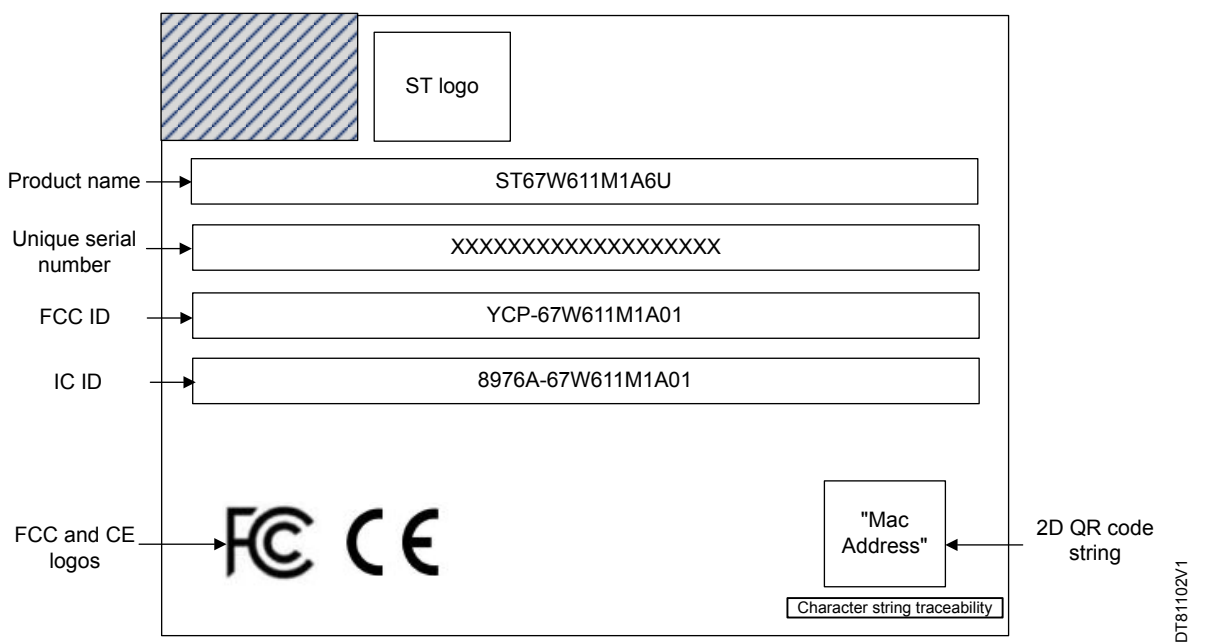
Figure 14. ST67W611M1A6U part marking
