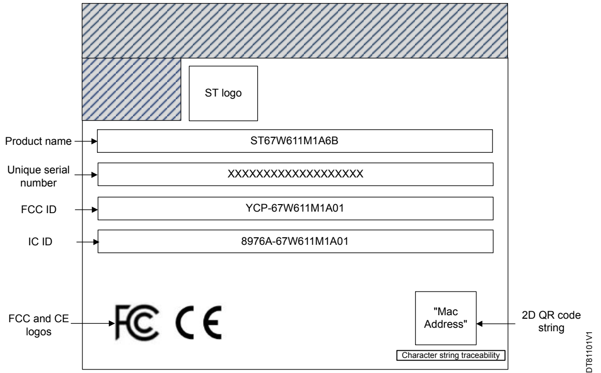
Figure 13. ST67W611M1A6B part marking
