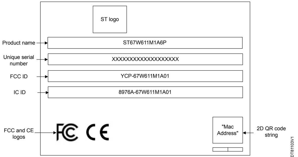
Figure 15. ST67W611M1A6P part marking
