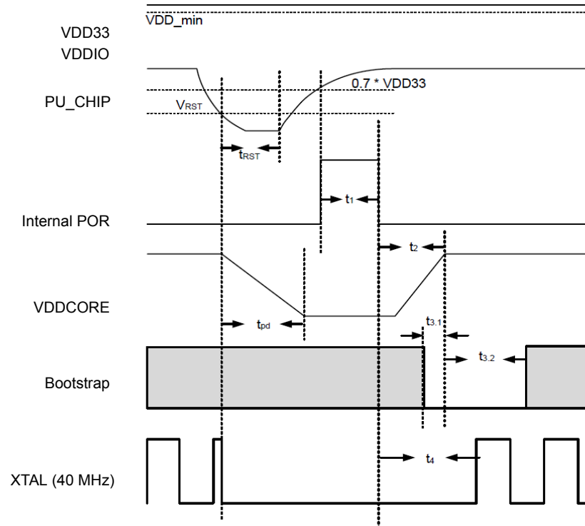
Figure 6. Shutdown sequence
