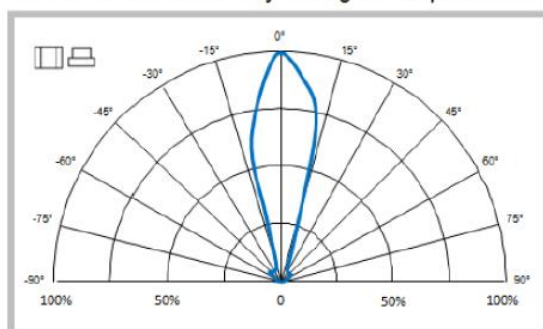
Relative Radiant Intensity vs Angular Displacement
