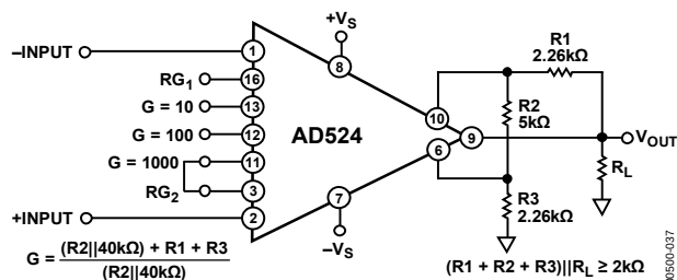
Figure 37. Gain of 2000
