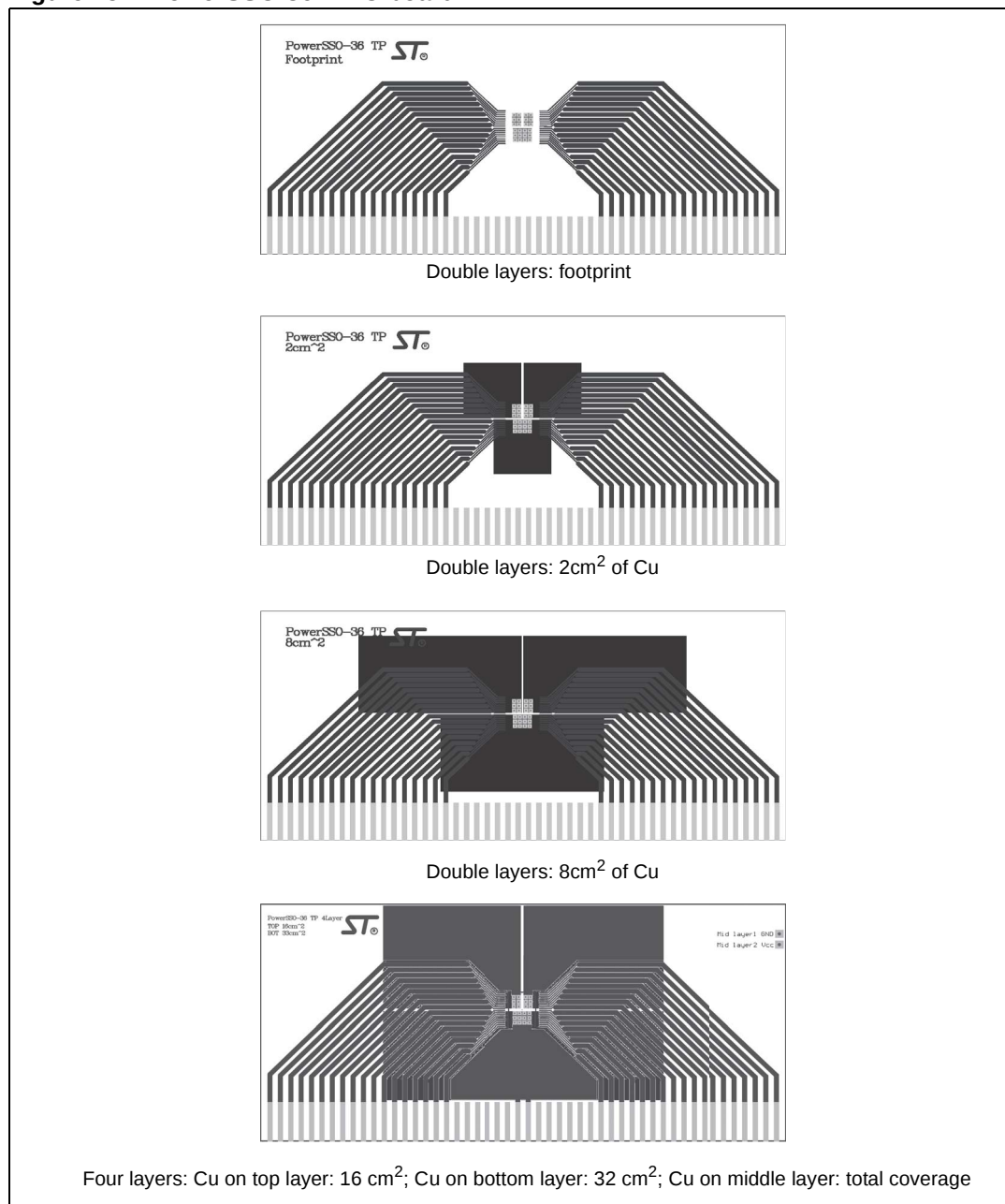
Figure 15. PowerSSO-36™ PC board
