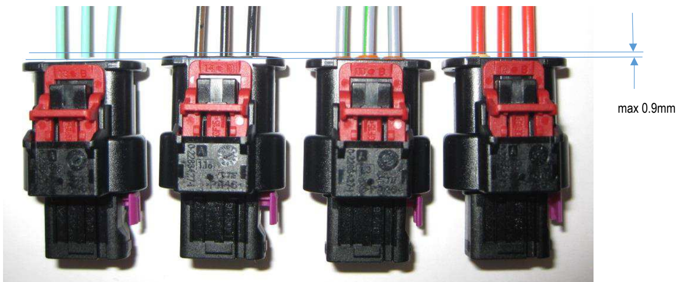
Figure 4: 3 posn, HPF 1.2, receptacle housing, radial seal Contact insertion of HPF 1.2 contact
