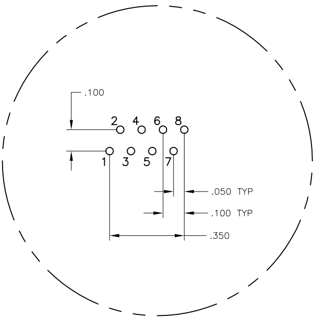
Pin Designations
