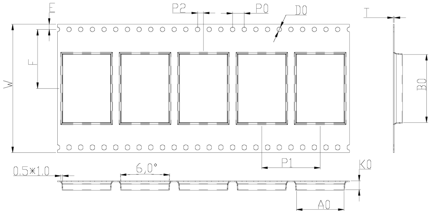
Figure 7 - Tape Specifications
