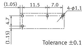
Recommended PC board pattern ( BOTTOM VIEW )
