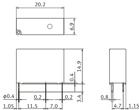
External dimensions
