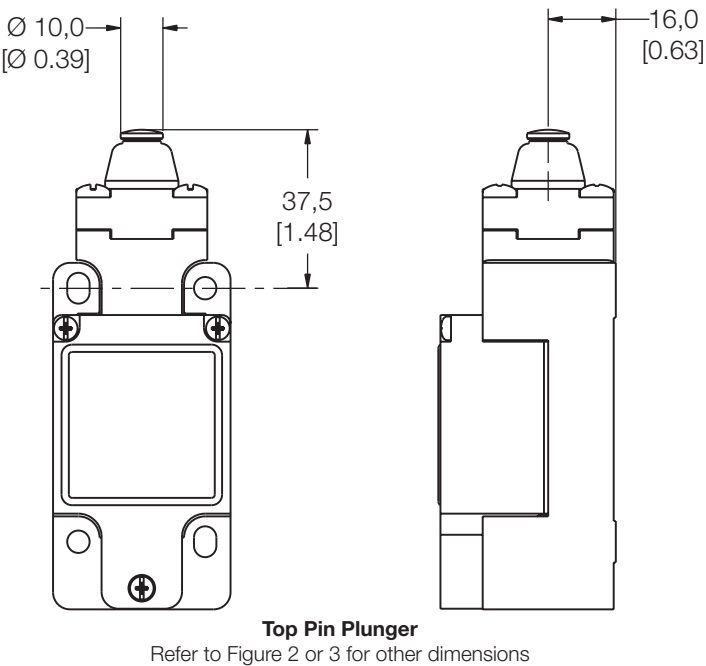
Figure 6. Pin Plunger Dimensions
