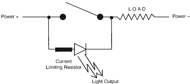
Figure 16. Wiring Diagram 1
