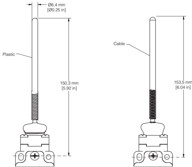
Figure 10. Plastic Rod and Flexible Cable
