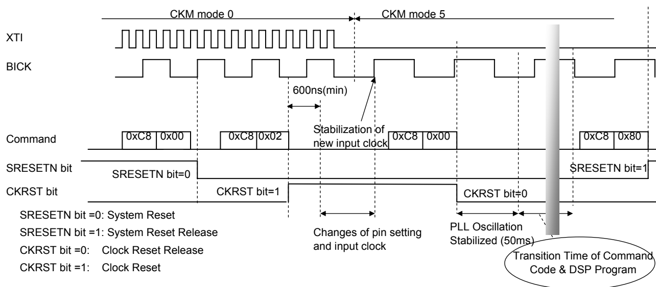
Figure 11. Clock Set Sequence (Ex: CKM Mode 0 → CKM Mode 5)
