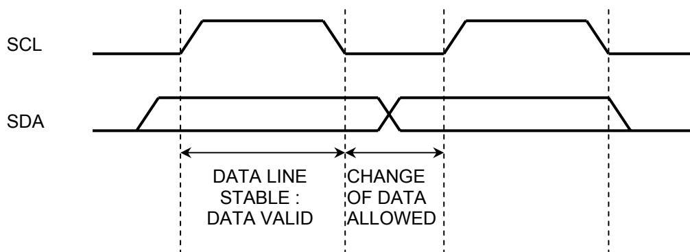
Figure 29. Data Transition
