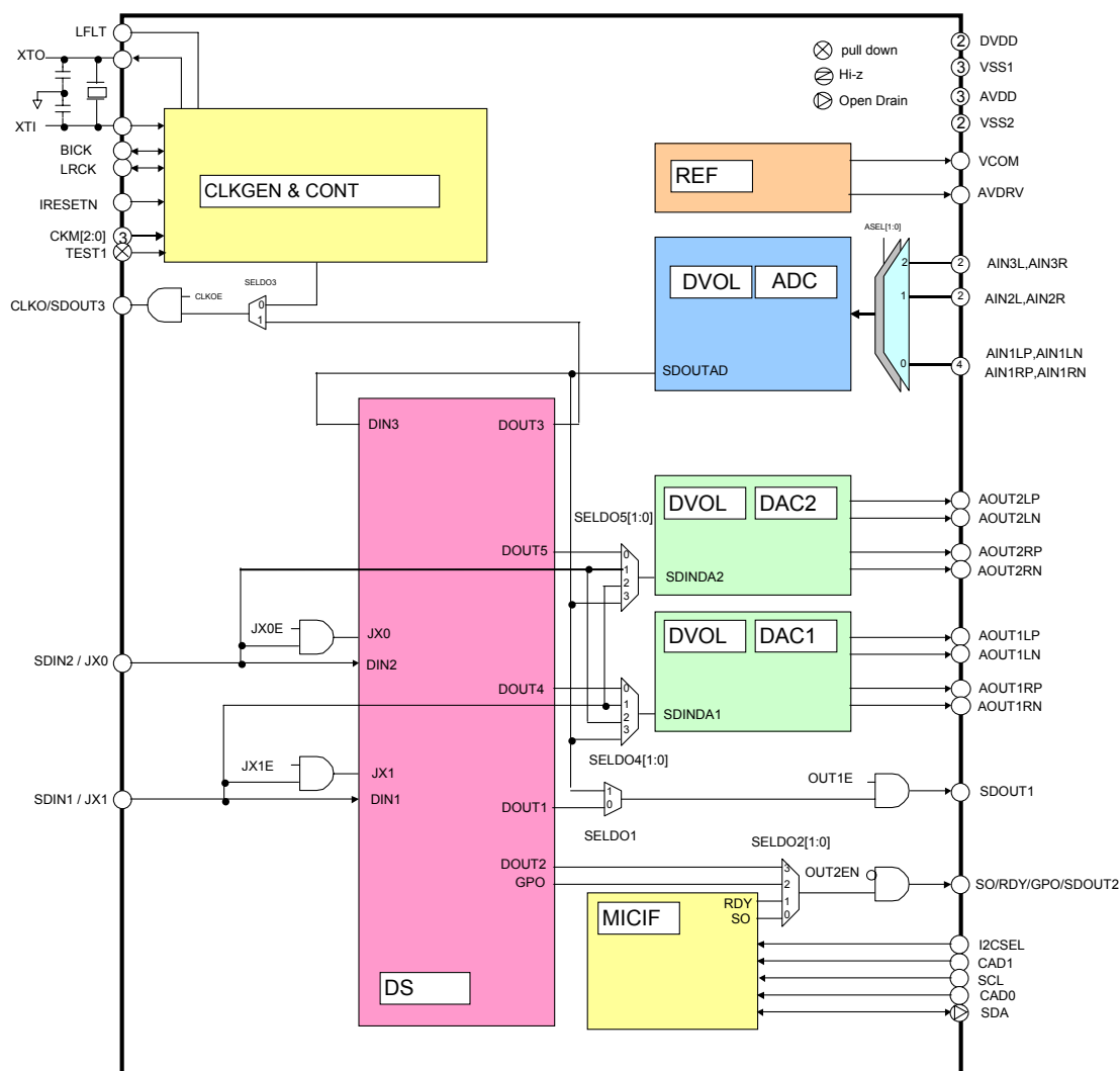
Figure 1. Block Diagram
