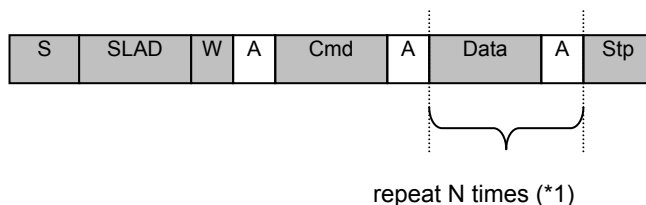
Figure 35. Write Sequence
