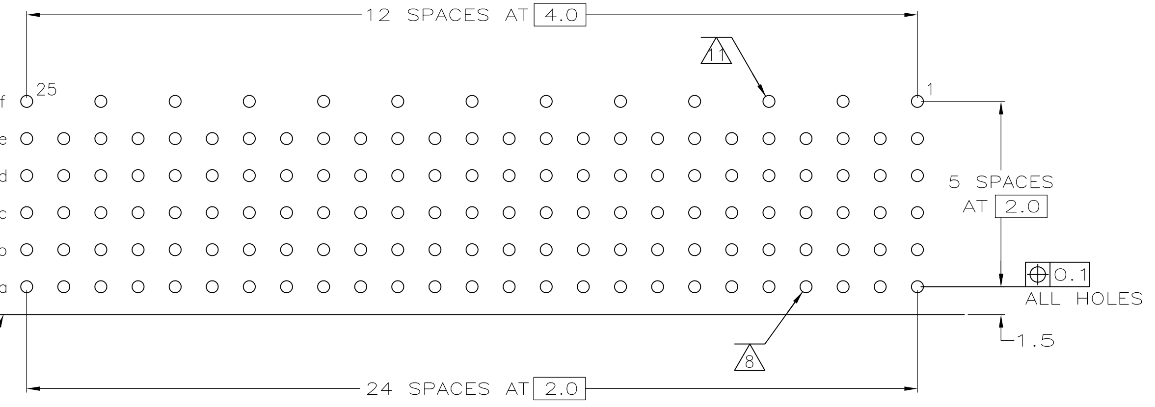
COMPONENT SIDE AS SHOWN RECOMMENDED PCB HOLE LAYOUT
