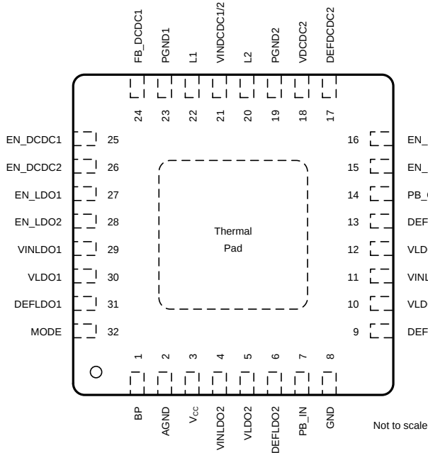
TPS65050 RSM Package 32-Pin VQFN With Exposed Thermal Pad Top View
