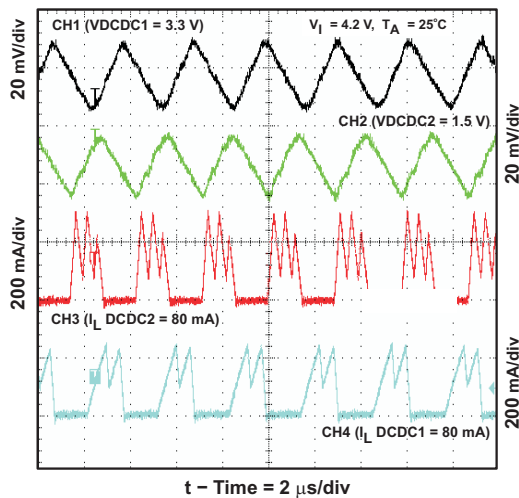
Figure 19. Output Voltage Ripple PWM/PM Mode = LOW
