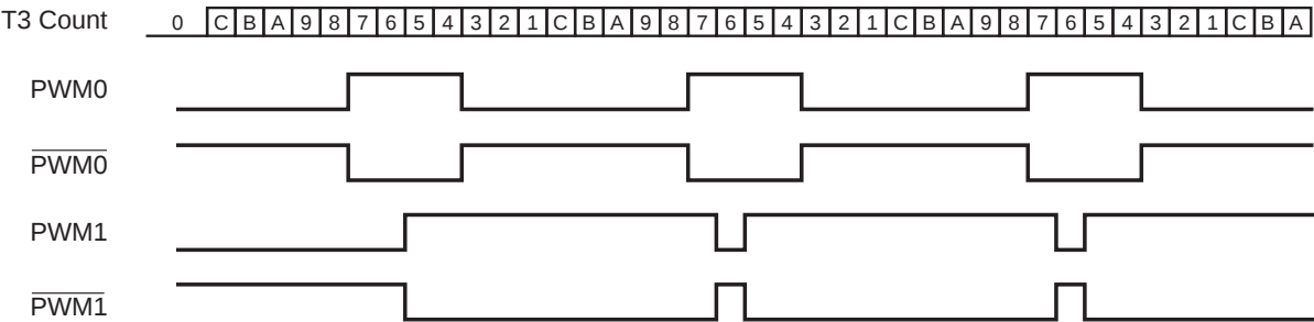
Figure 31. Multi-PWM Operation
