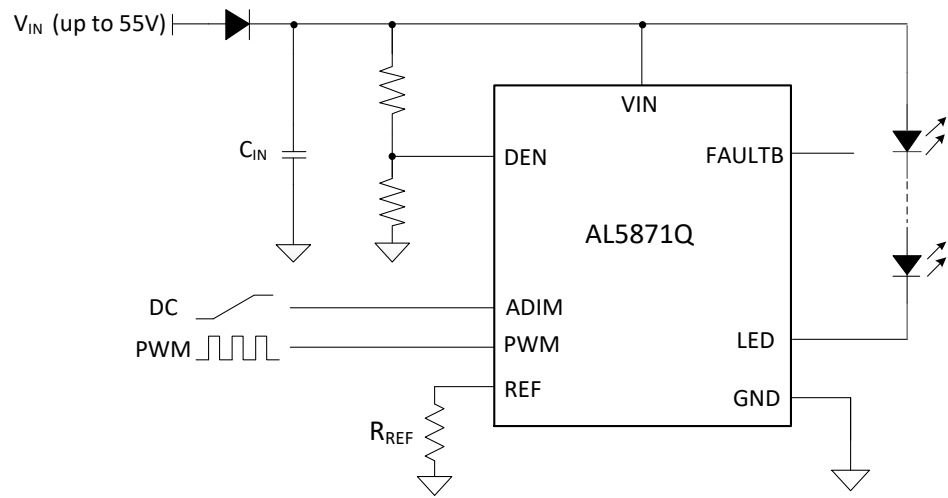
Figure 1. Typical Application
