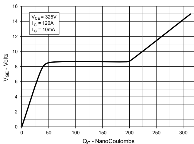
Fig. 8. Gate Charge
