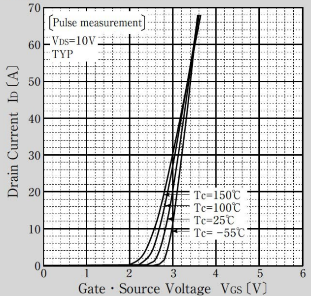
Transfer Characteristics
