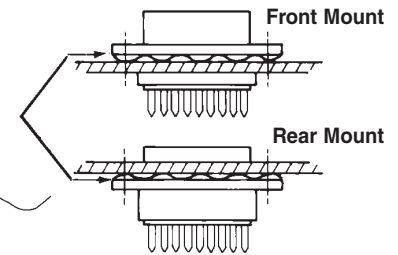
Waved Metal Grounding/Shielding Gasket (shown in free state)
