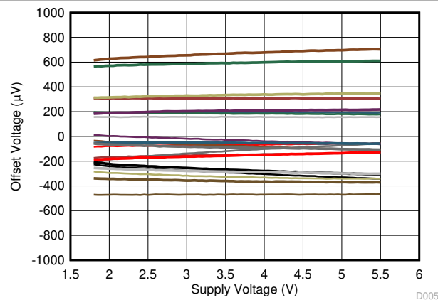
Figure 7-5. Offset Voltage vs Supply Voltage
