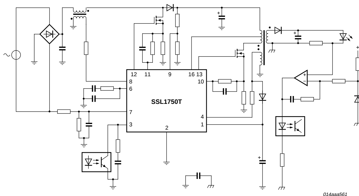
Fig 3. Application circuit
