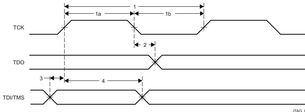
Figure 7-109. JTAG Timing
