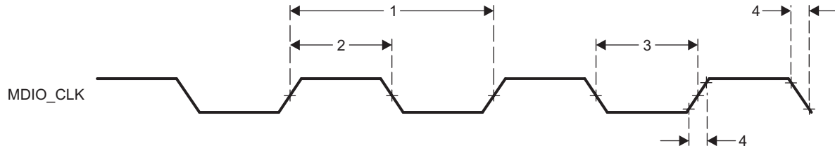
Figure 7-102. PRU-ICSS MDIO_CLK Timing
