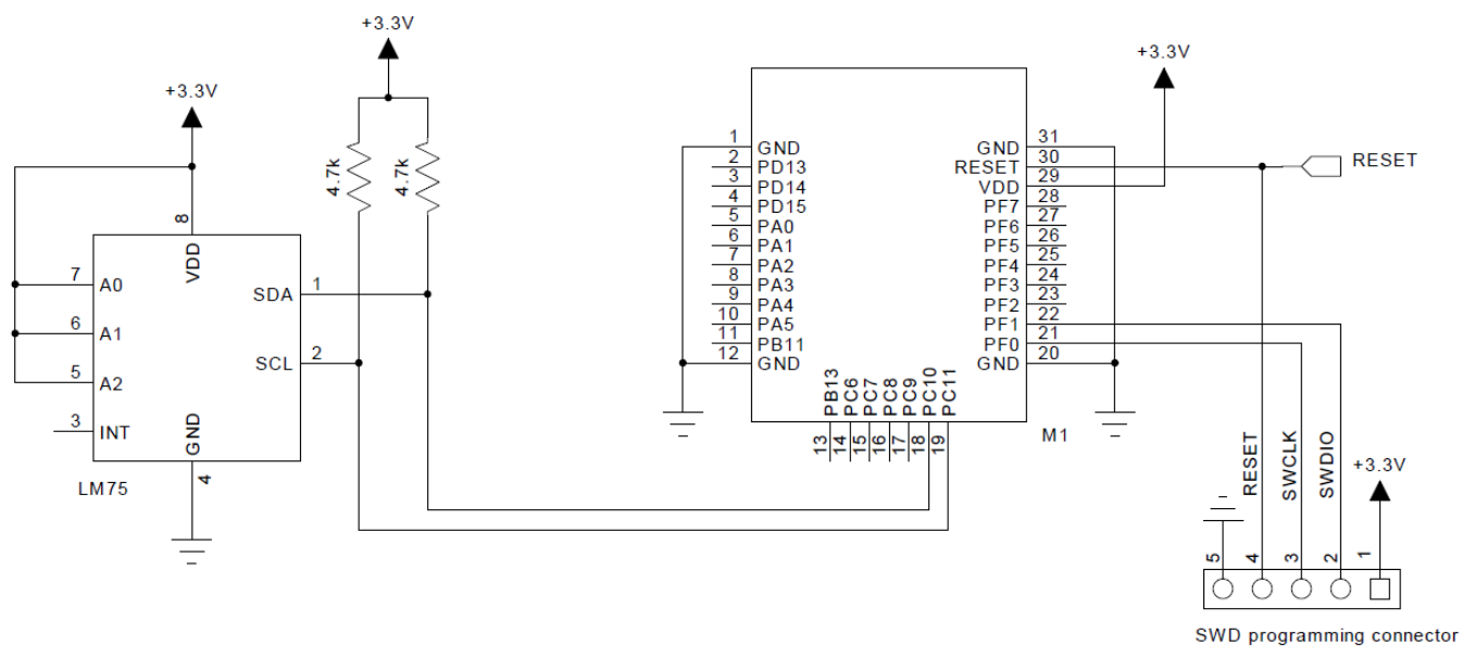
Figure 5.3. ARTIK 020 Module Connected with I 2 C Device
