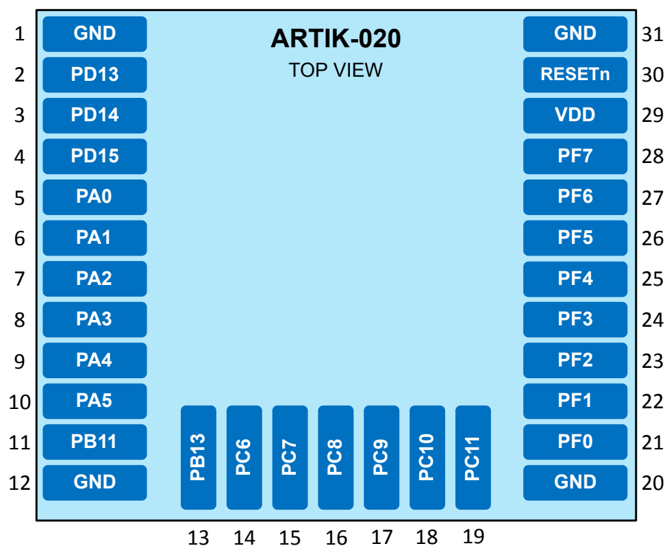
Figure 7.1. ARTIK 020 Pinout
