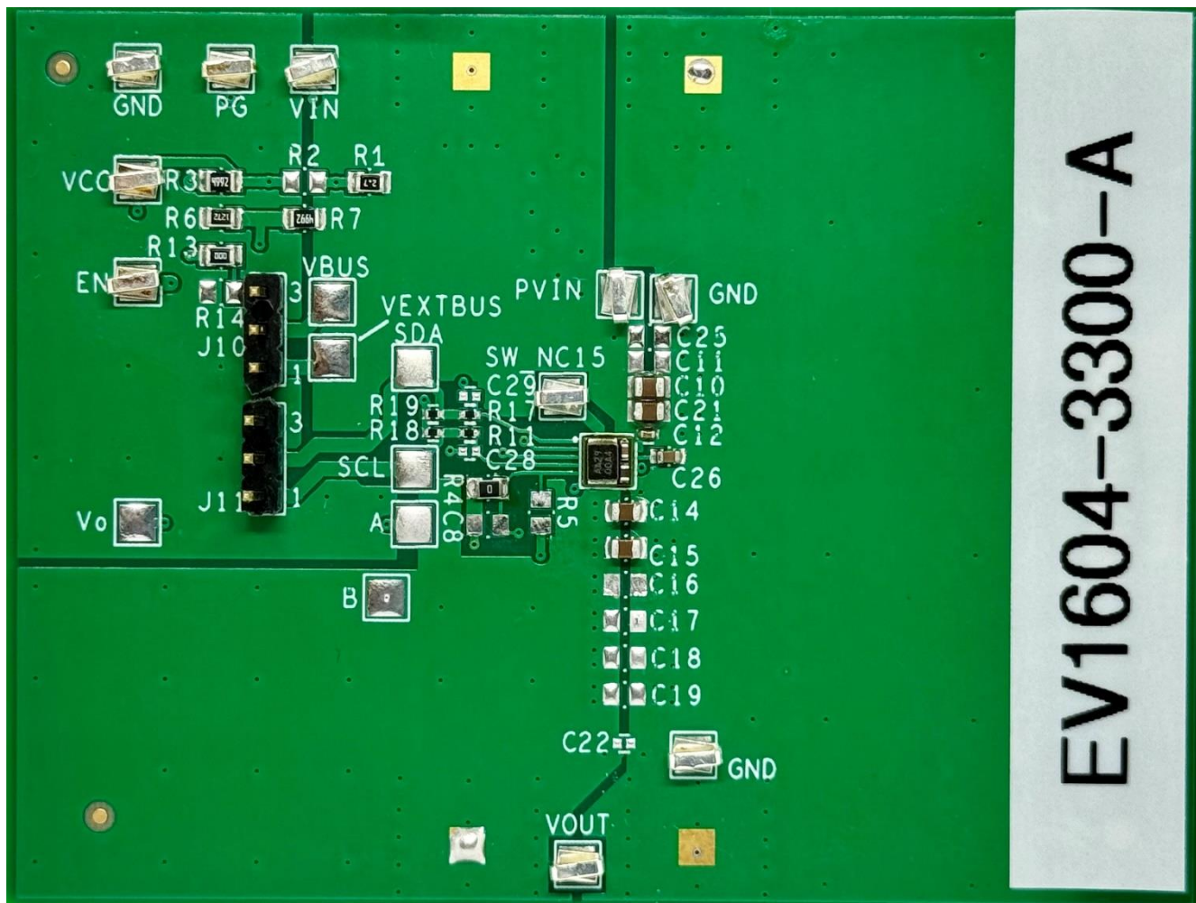
Figure 1 Board layout
