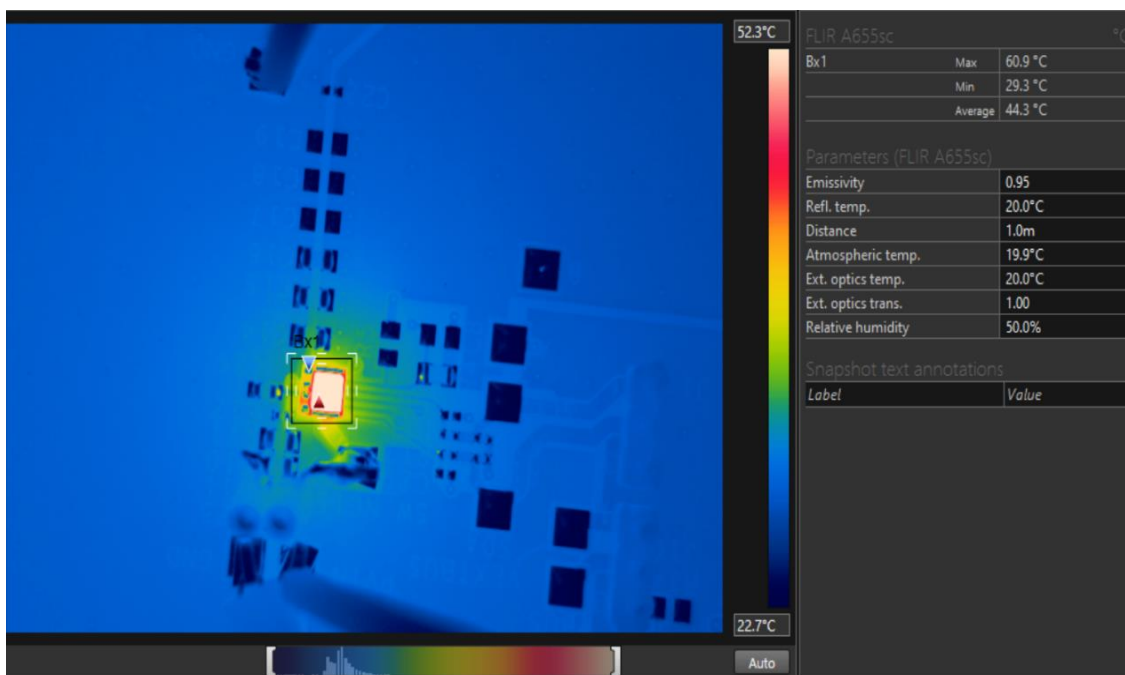
Figure 18 Thermal image( P_{VIN}=12V , I_{OUT}=4A ) – maximum temperature rise = 38^{\circ}C
