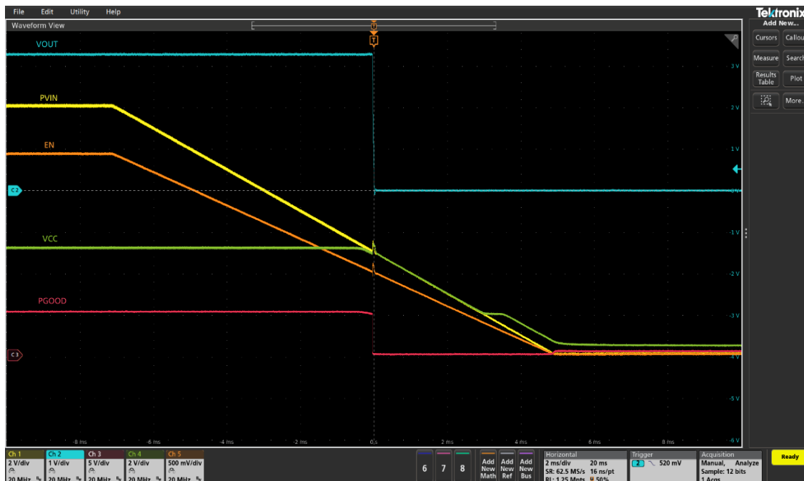
Figure 5 Shutdown with Enable de-assertion at 4A load (Ch1:PV IN , Ch2: V OUT , Ch3: PG, Ch4:V CC , Ch5: Enable)
