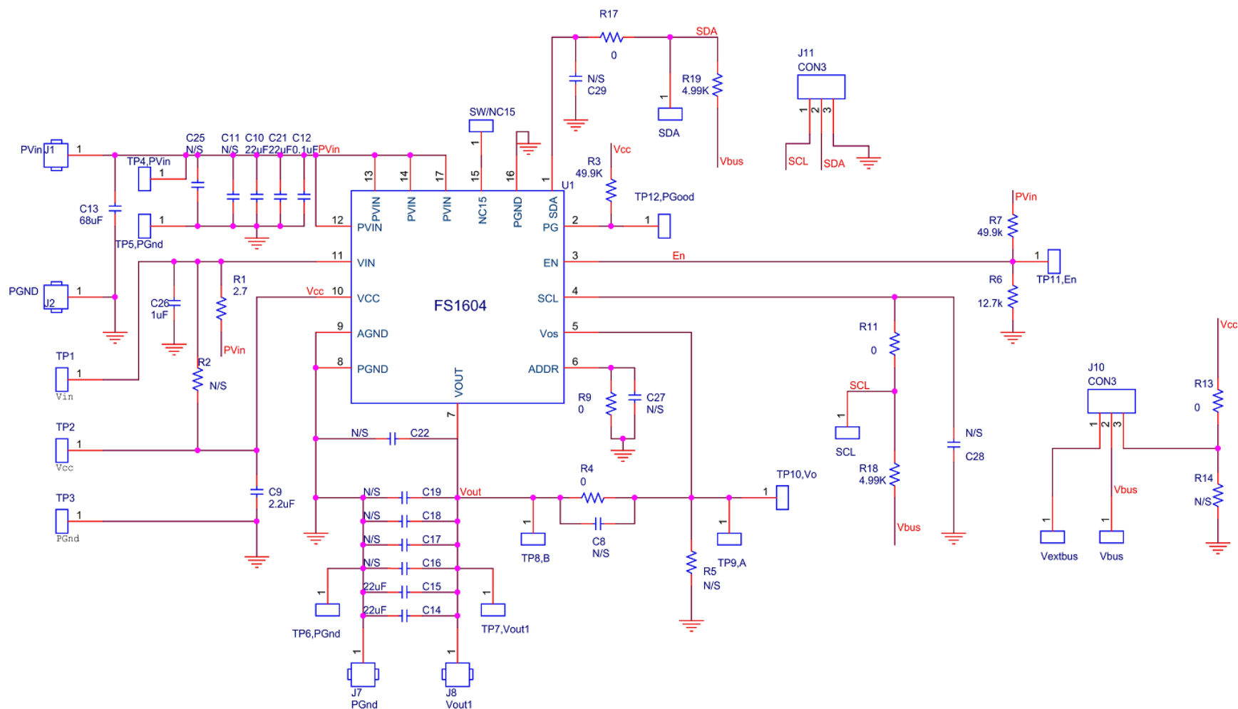
Figure 2 Schematic
