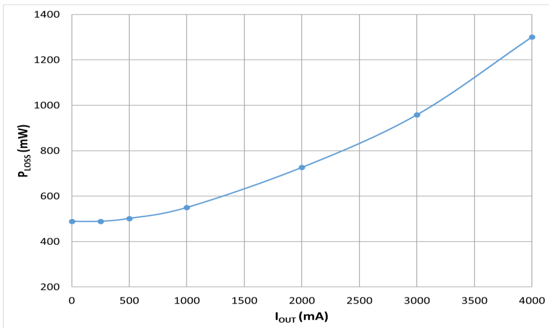
Figure 16 Power loss
