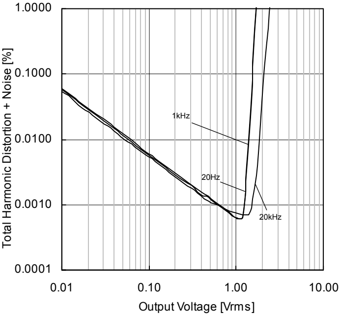
Figure 52. Total Harmonic Distortion + Noise vs Output Voltage (V + =5V, R L =2kΩ, T A =25°C)
