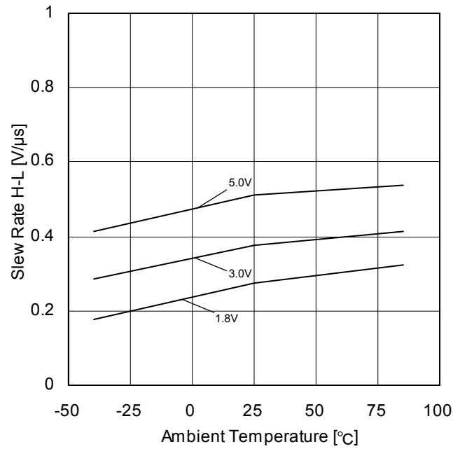
Figure 75. Slew Rate H-L vs Ambient Temperature ( R_L=2k\Omega )
