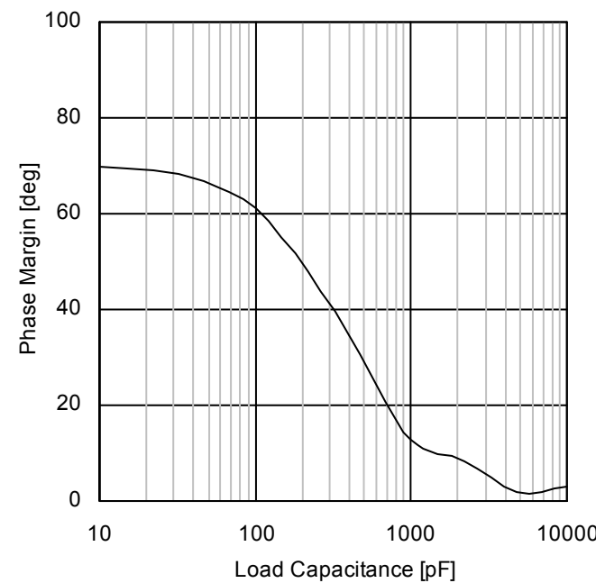
Figure 24. Phase Margin vs Load Capacitance ( V_+=5V , T_A=25^\circ C )
