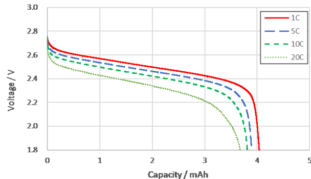
Discharge characteristics
