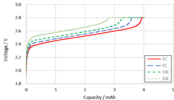
Charge characteristics
