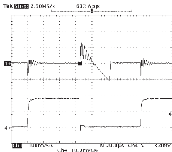
Fig. 16: Load Step Response 0mA to 800mA V_{\text{IN}}=3.3\text{V} , V_{\text{OUT}}=1.8\text{V} , C_{\text{IN}}=10\mu\text{F} , C_{\text{OUT}}=2.2\mu\text{F} , Ceramic Signal 1= V_{\text{OUT}} , Signal 4= I_{\text{LOAD}}
