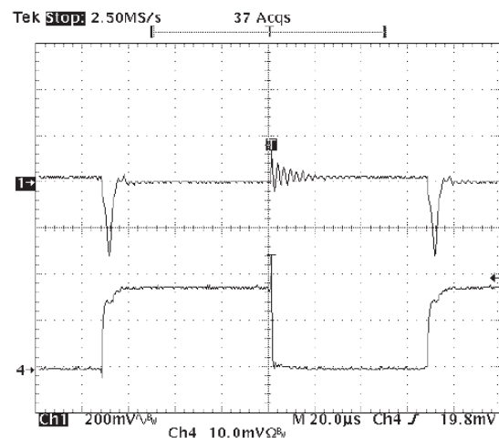
Fig. 17: Load Step Response 0mA to 800mA V_{\text{IN}}=3.3\text{V} , V_{\text{OUT}}=1.8\text{V} , C_{\text{IN}}=10\mu\text{F} , C_{\text{OUT}}=2.2\mu\text{F} , OSCON Signal 1= V_{\text{OUT}} , Signal 4= I_{\text{LOAD}}
