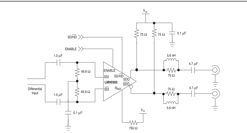
Figure 2-13. SDI Cable Driver
