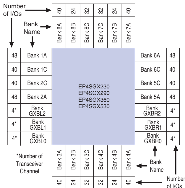
Figure 2–2. EP4SGX530KH40 Device I/O Bank Diagram
