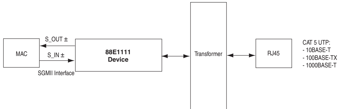
Figure 2–10. SGMII Interface between FPGA (MAC) and Marvell 88E1111 PHY
