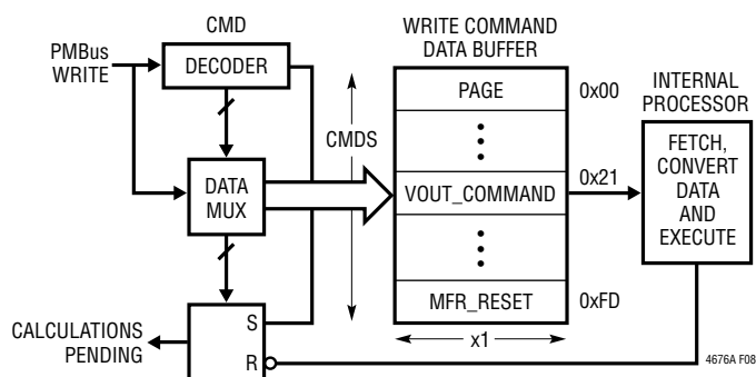
Figure 8. Write Command Data Processing
