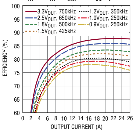
Efficiency vs Output Current, 24\text{V}_{\text{IN}} , \text{V}_{\text{OUT}0} and \text{V}_{\text{OUT}1} Paralleled, \text{V}_{\text{IN}} = \text{SV}_{\text{IN}} = \text{V}_{\text{IN}n} , \text{INTV}_{\text{CC}} Open
