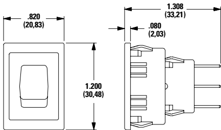
B2 Recessed Snap-in Actuator Guard, Black
