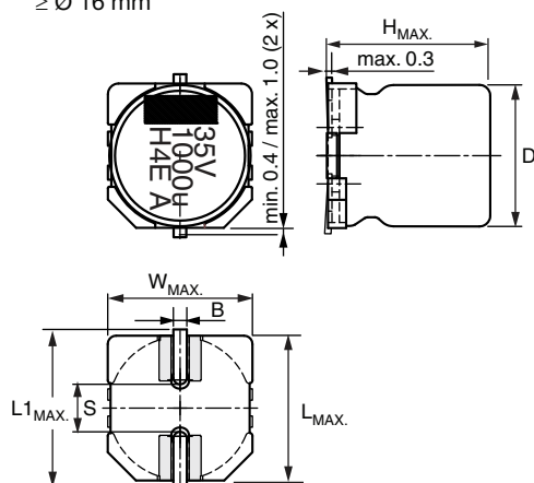
Fig. 2 - Dimensional outline
