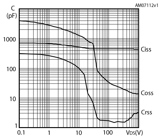
Figure 8: Capacitance variations
