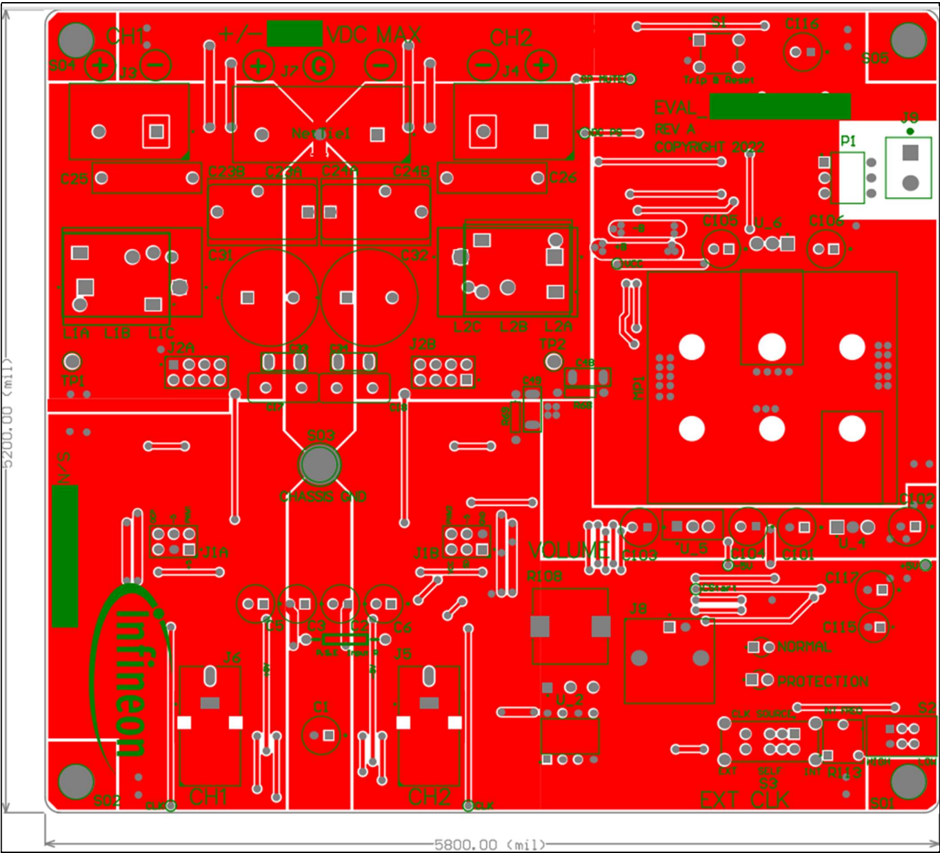
Figure 20 Motherboard top view
