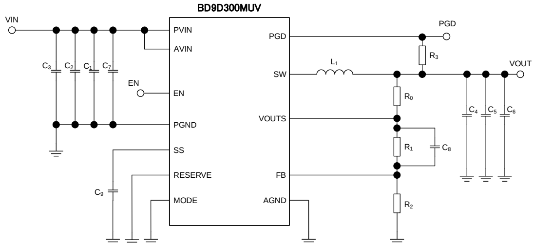
Figure 45. Application Circuit
