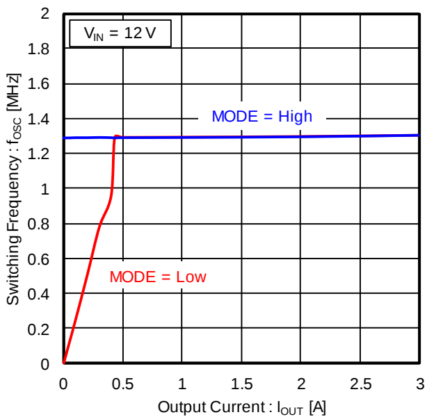
Figure 19. Switching Frequency vs Output Current ( V_{IN} = 12\text{ V} , V_{OUT} = 5\text{ V} )
