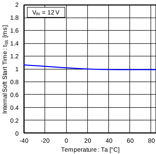
Figure 17. Internal Soft Start Time vs Temperature
