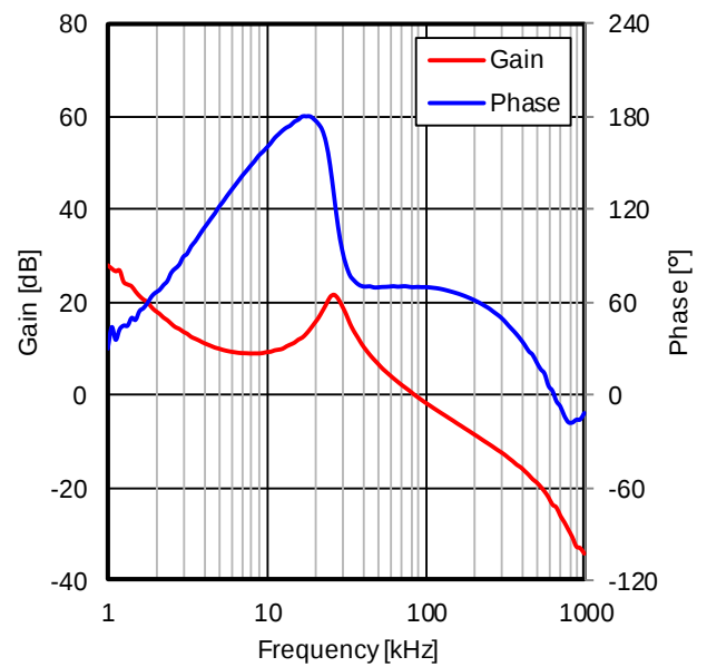
Figure 37. Frequency Characteristics I_{OUT} = 2.0\text{ A}
