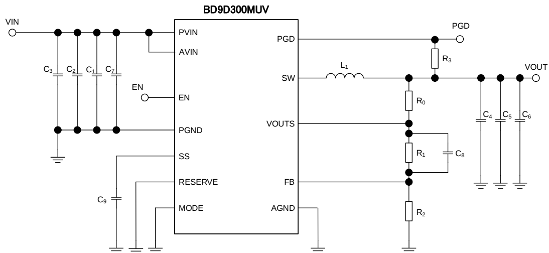
Figure 35. Application Circuit
