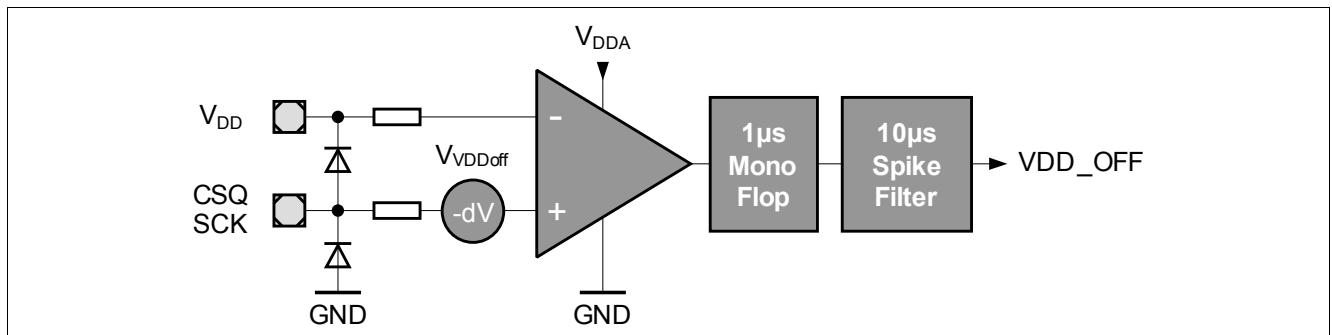
Figure 4-17 V_{DD} - off comparator
