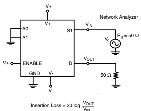
Figure 5. Insertion Loss
