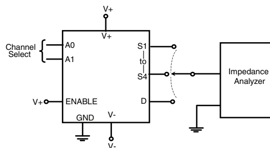
Figure 8. Source/Drain Capacitance
