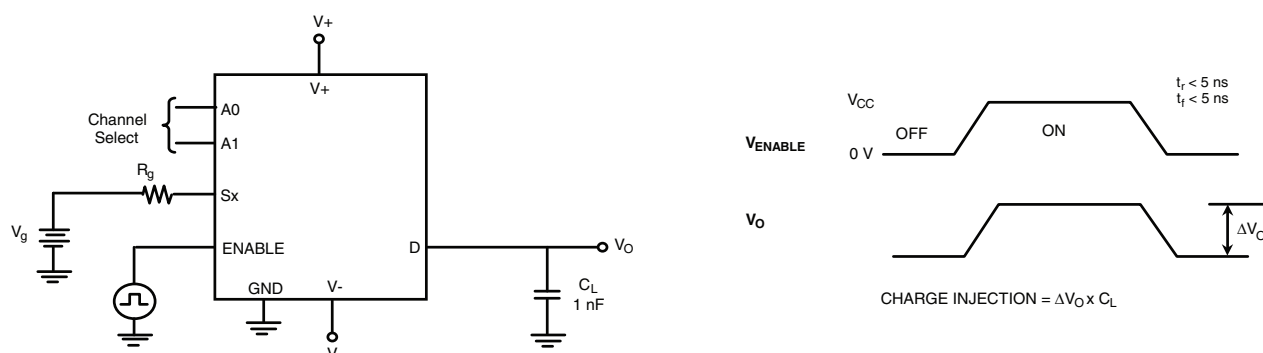
Figure 4. Charge Injection
