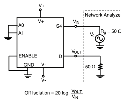
Figure 6. Off-Isolation
