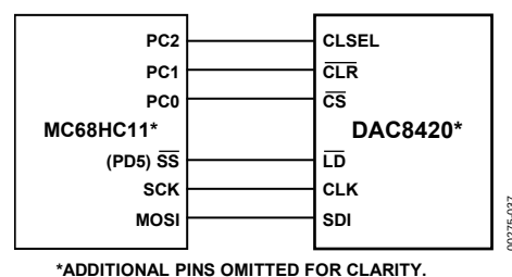
Figure 37. MC68HC11 Microcontroller Interface
