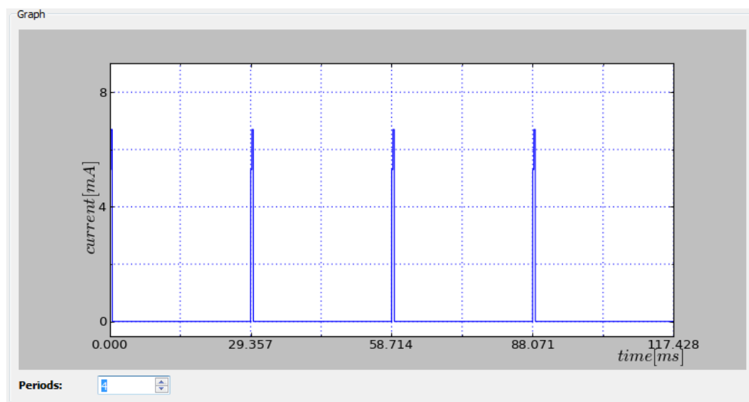
Figure 28. Current graph
