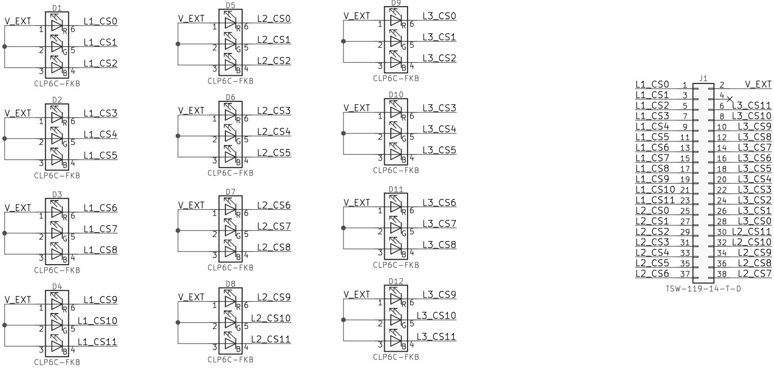
Figure 4. STEVAL-LLL007D2 circuit schematic
