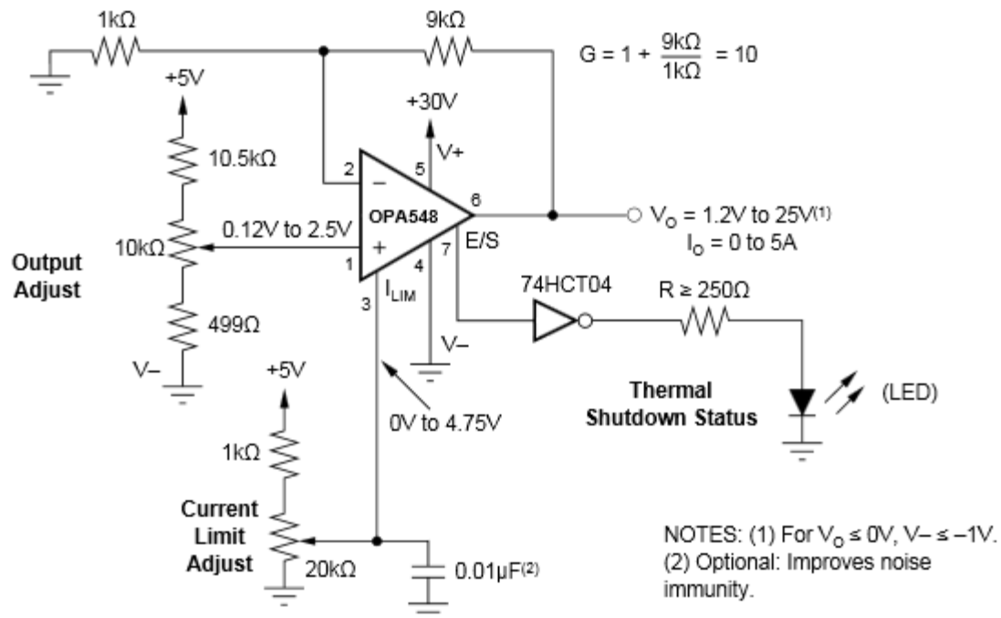
Figure 31. Resistor-Controlled Programmable Power Supply Schematic
