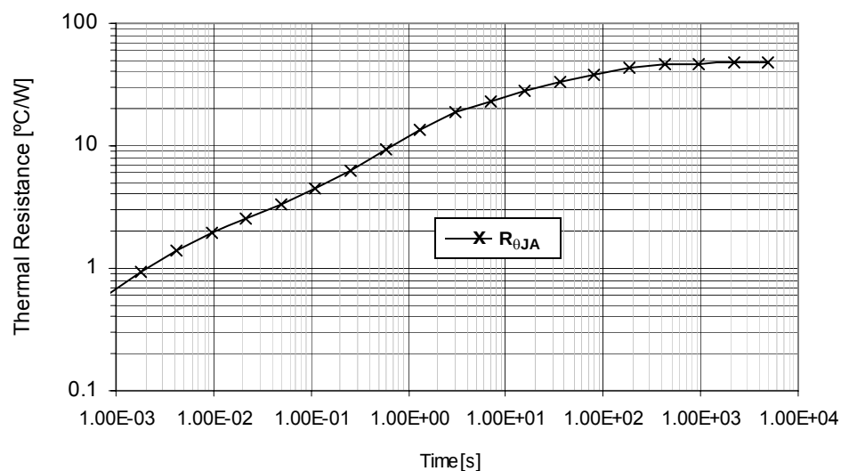
Figure 41. Transient Thermal Resistance R_{\theta JA} , 1 W Step response, Device on Thermal Test Board Area A = 600 (mm²)
