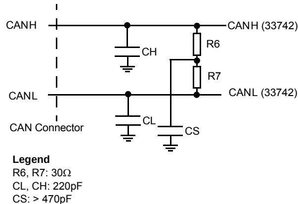
Figure 37. CAN Bus Split Termination
