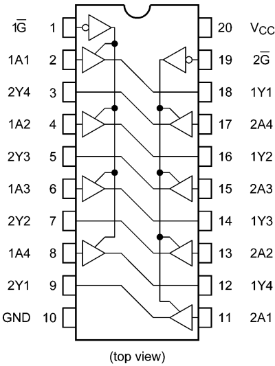
74VHCT244AFT
