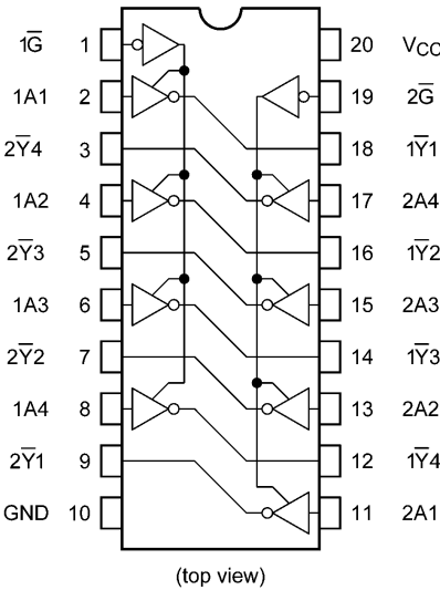
74VHCT240AFT
