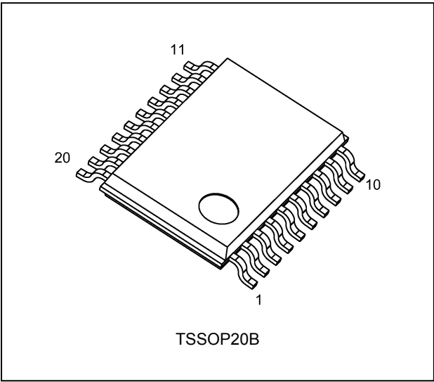
74VHCT244AFT
