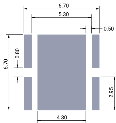
Recommended Soldermask Opening
