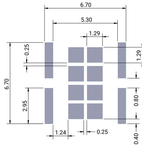
Recommended Stencil Opening
