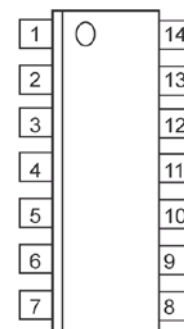
Top Viewing Pin Layout
