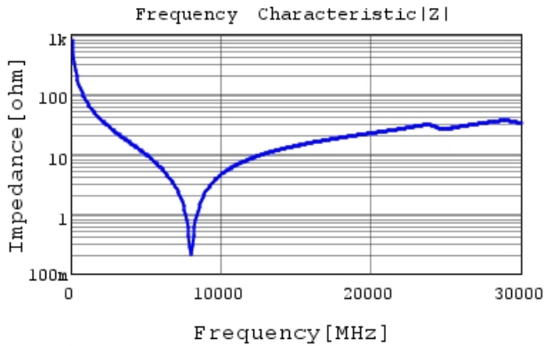
GJM0335C2A2R0WB01 |Z| DCOV, 25degC
