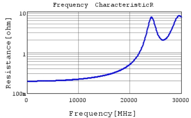
GJM0335C2A2R0WB01 R DCOV, 25degC
