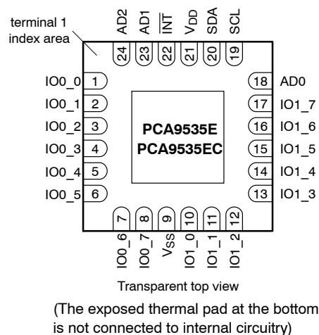
Figure 4. WQFN24
