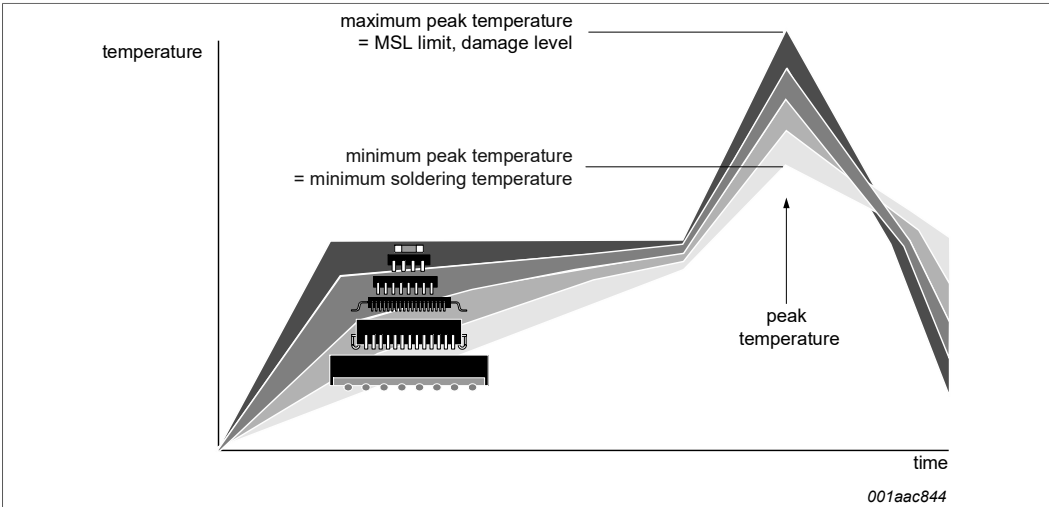
MSL: Moisture Sensitivity Level Figure 9. Temperature profiles for large and small components
