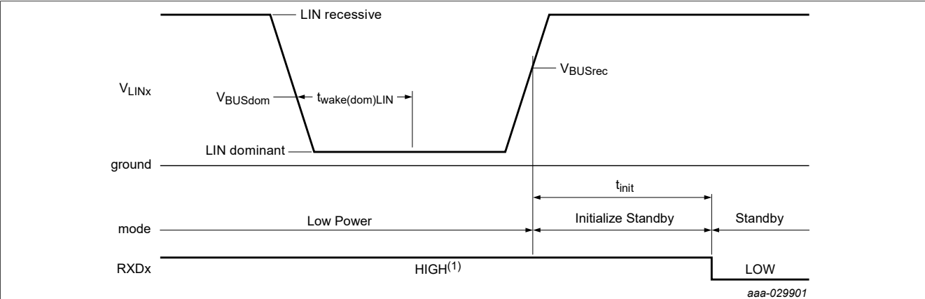
Figure 4. Principle of remote wake-up via LIN bus in Low Power mode
