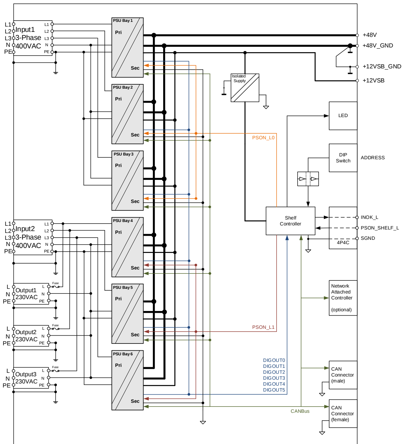
Figure 1. SPSTET4 Block Diagram
