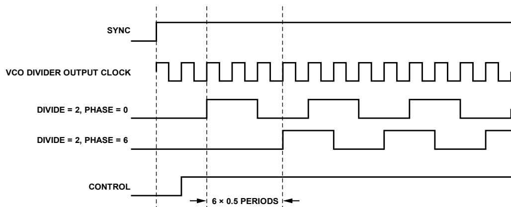
Figure 30. Clock Output Synchronization Timing Diagram
