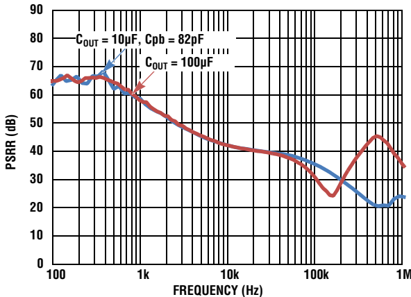
FIGURE 13. PSRR vs FREQUENCY AND OUTPUT CAPACITANCE ( I_{OUT} = 100mA )
